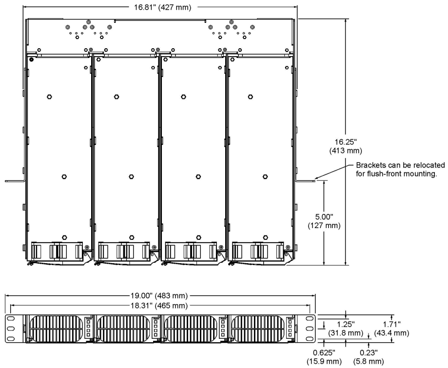
Package Outline
